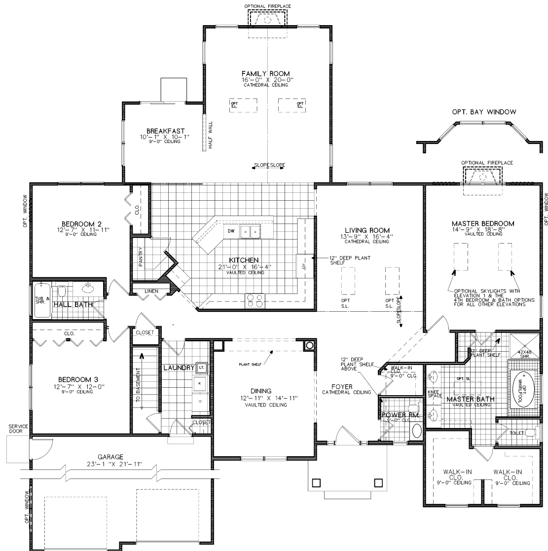
FIRST-FLOOR PLAN
