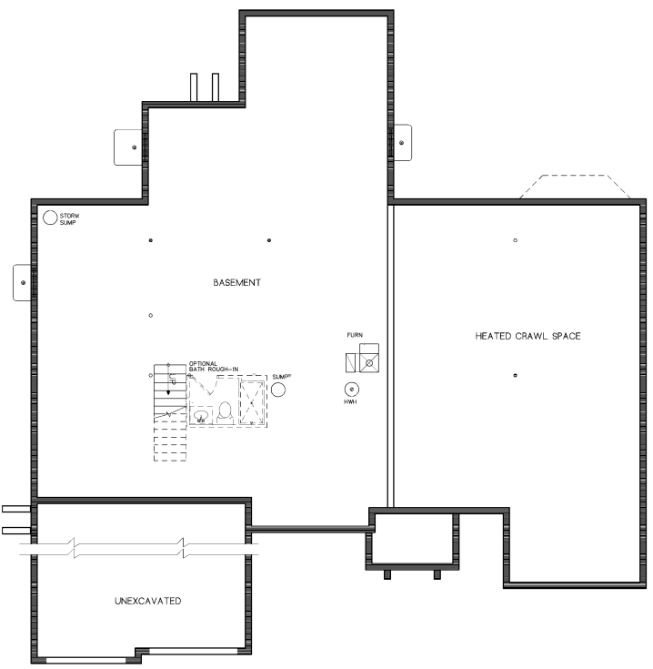
BASEMENT / CRAWL PLAN
