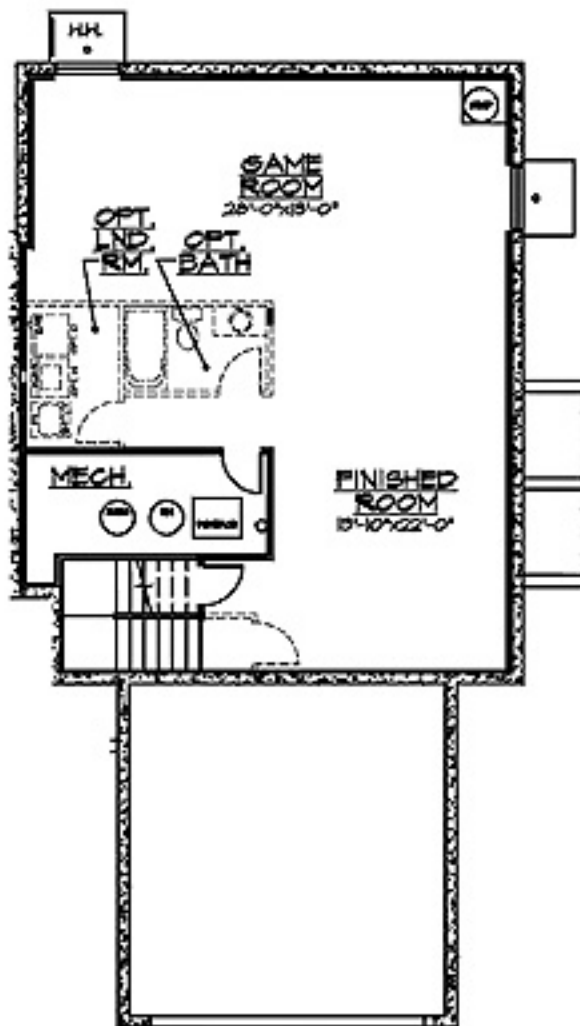
OPT FINISHED BASEMENT PLAN
