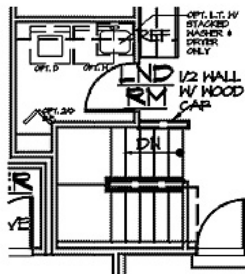
OPTIONAL OPEN BASEMENT STAIR UNIT D
