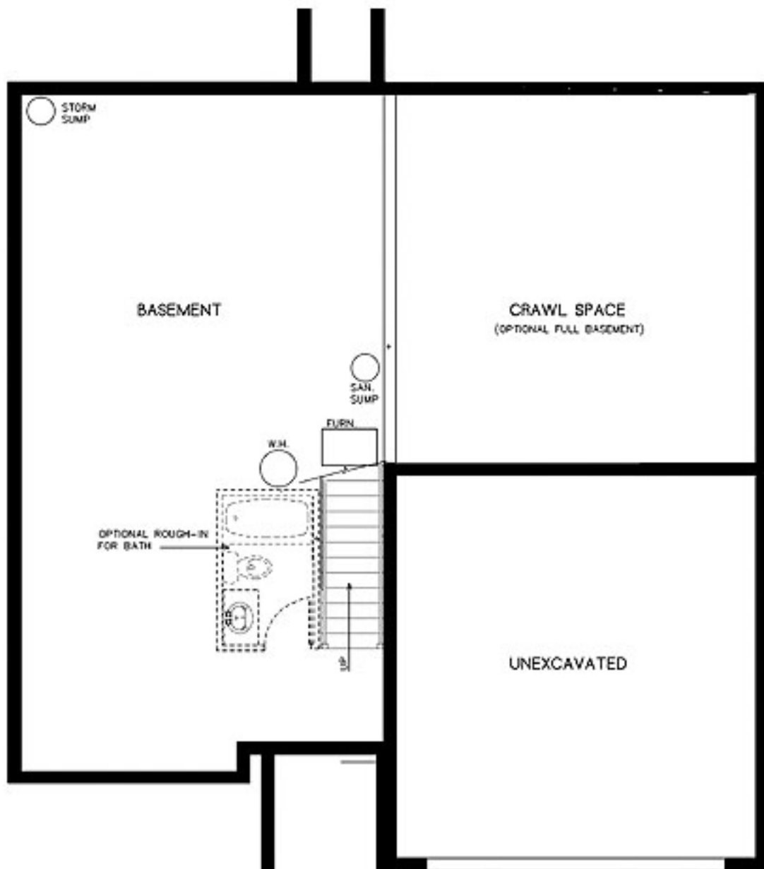
BASEMENT\CRAWL PLAN
