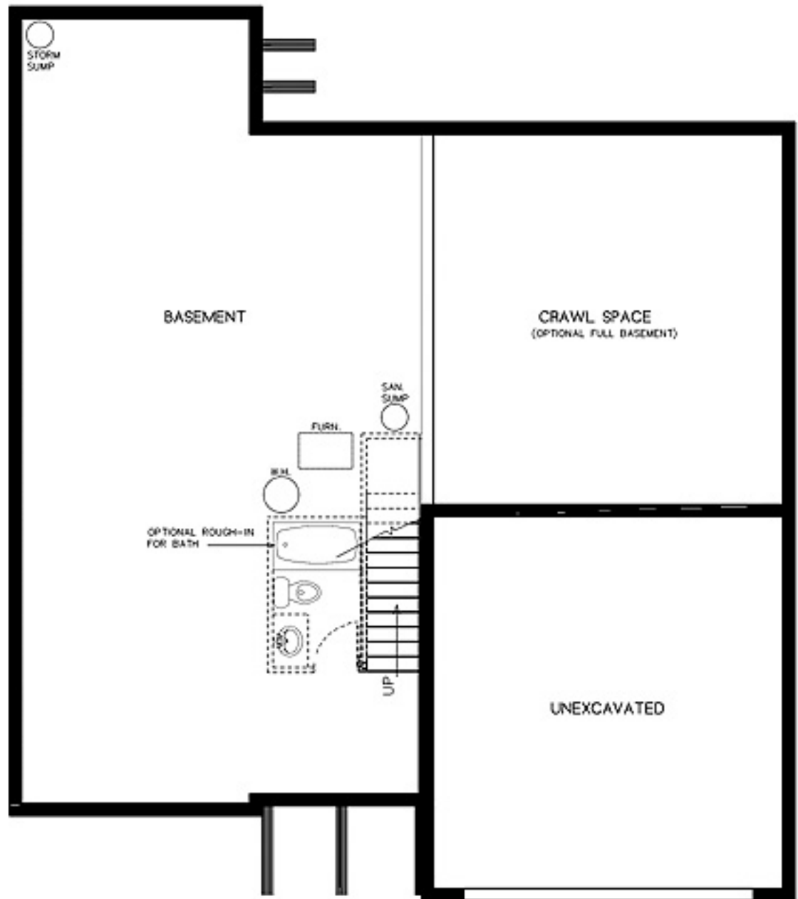
BASEMENT\CRAWL PLAN
