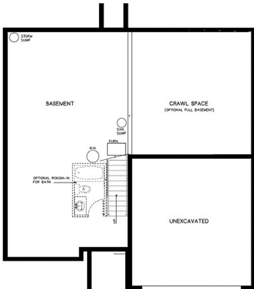
BASEMENT \ CRAWL PLAN
