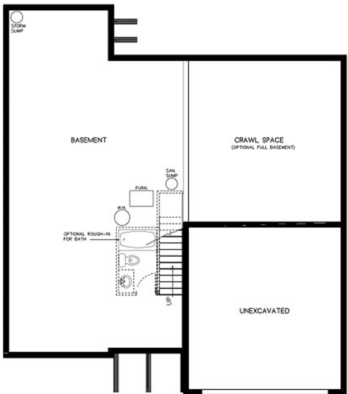
BASEMENT\CRAWL PLAN
